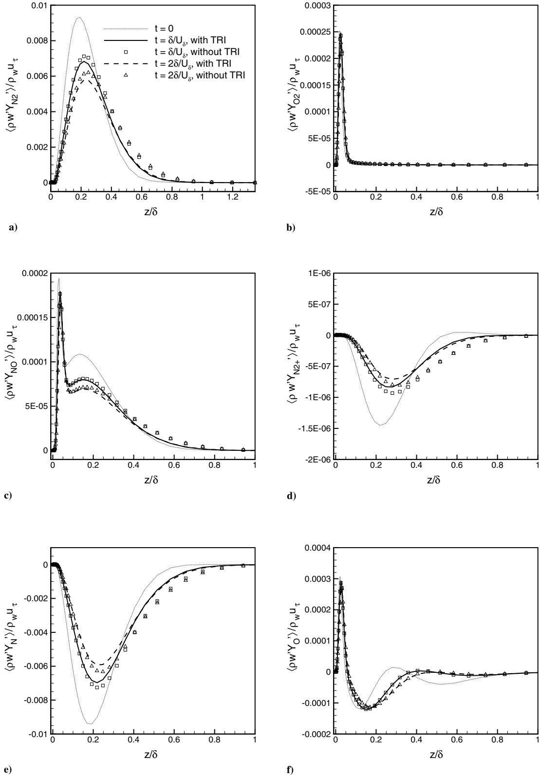
Fig. 12 Time evolution of turbulent mass flux \overline{\rho w' Y_i'} / \bar{\rho}_w u_\tau for case II (with emission TRI) and case III (without emission TRI): a) N_2 , b) O_2 , c) NO , d) N_2^+ , e) N , and f) O .
