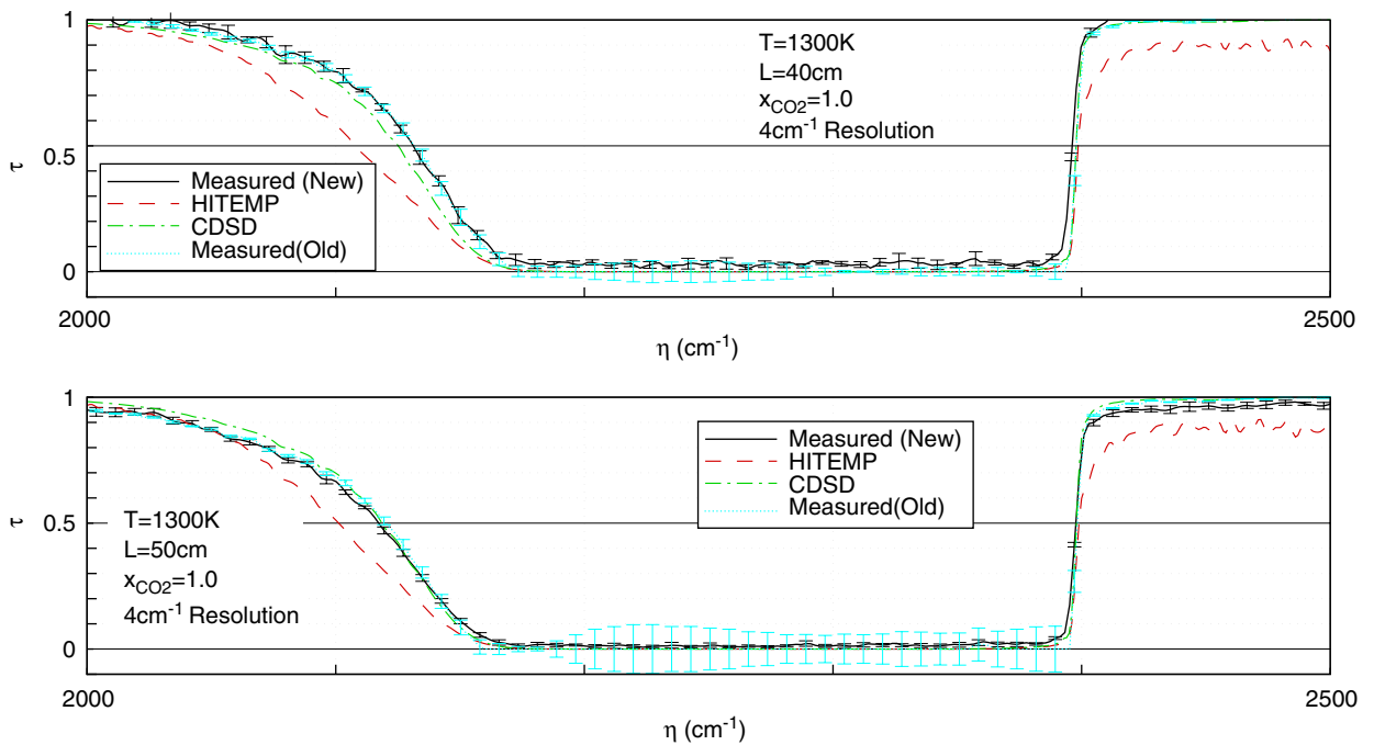
Fig. 9. Comparison of experimental data with HITEMP and CDSD (1300 K, 4.3 \mu m band of CO 2 ).
