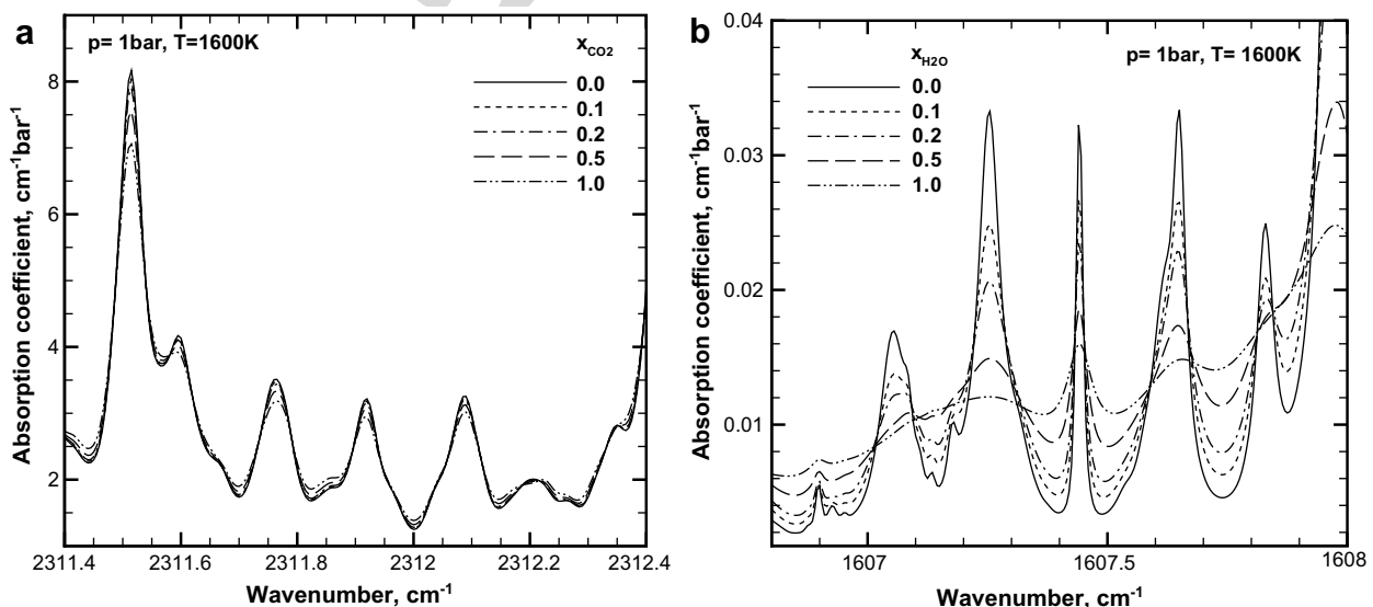
Fig. 2. Pressure-based absorption coefficient in a small spectral interval (obtained from Wang and Modest [27]): (a) CO 2 and (b) H 2 O.
